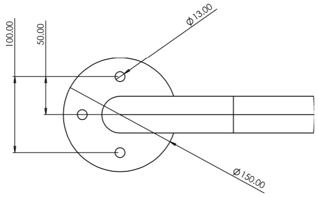
DETAIL A SCALE 2:5
